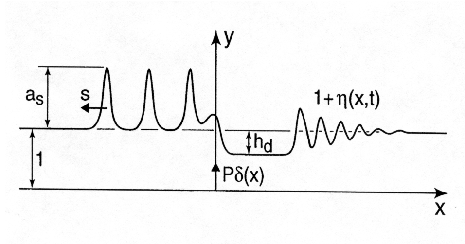
Figure 1: An illustration of the schematic solution \eta(x, t) of fKdV for a fixed time t .
