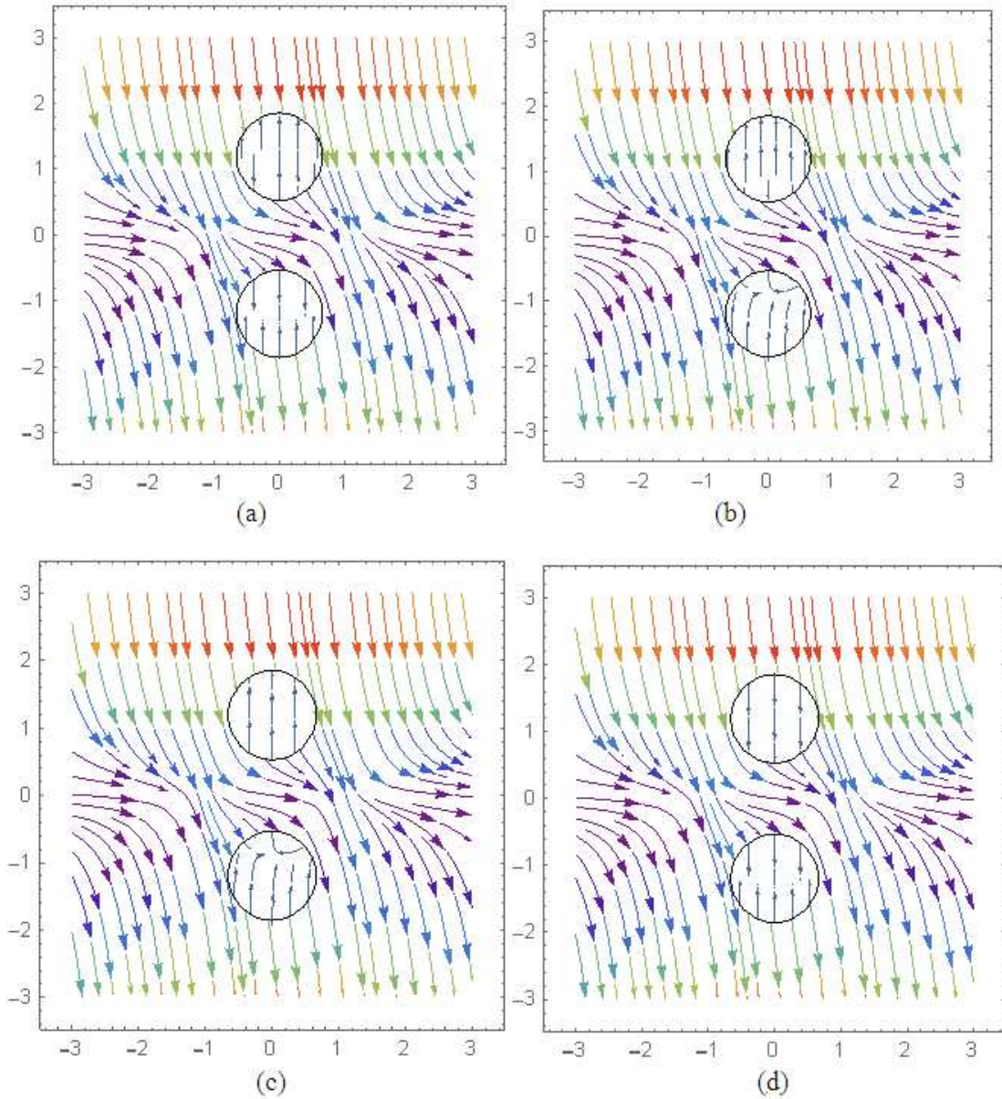
Figure 5: Plot of Streamlines in the xy - plane for \xi_1 = 1.2, \xi_2 = -1.2 , (a) \lambda_1 = 0.1, \lambda_2 = 0.1 (b) \lambda_1 = 10, \lambda_2 = 10 (c) \lambda_1 = 0.1, \lambda_2 = 10 (d) \lambda_1 = 10, \lambda_2 = 0.1
