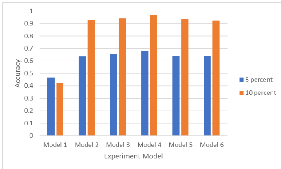
Figure 5: Accuracy comparison between models
