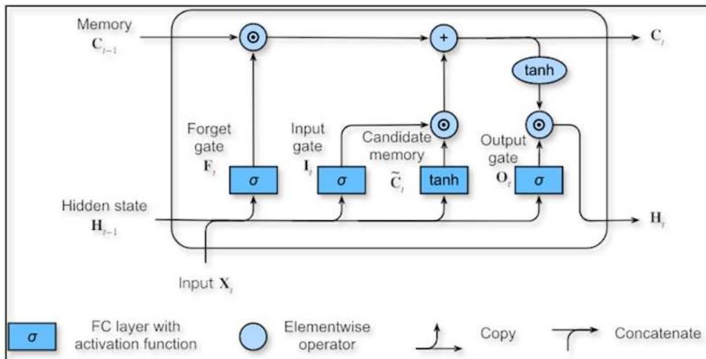
Figure 4: Hidden State
