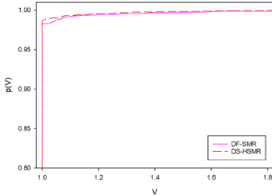
Figure 3: Performance profiles based on number of function evaluations (NFE).
