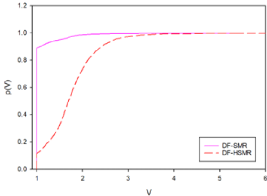
Figure 4: Performance profiles based on CPU time (in seconds).
