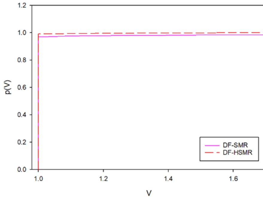
Figure 2: Performance profiles based on number of iterations (NOI).
