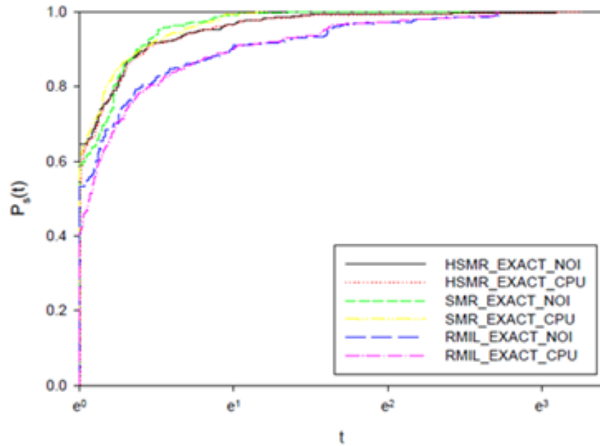
Figure 1: Performance Profile for SMR, HSMR, and RMIL.
