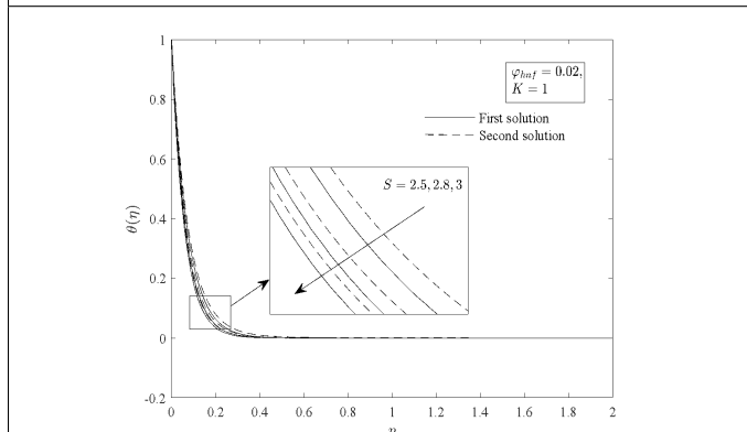
Figure 13: \theta(\eta) for varies S
