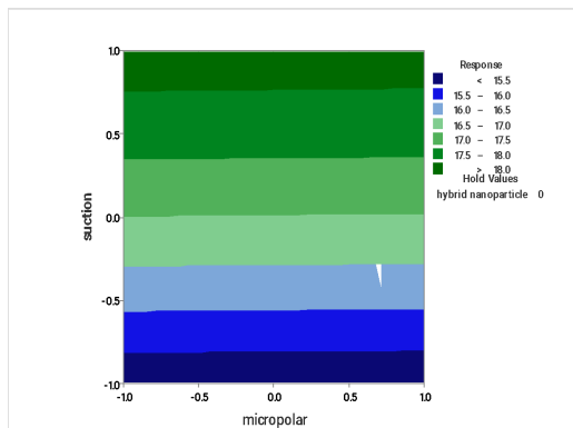
Figure 17: The interaction effect of hybrid nanoparticle, micropolar and suction on Nu_x Re_x^{-1/2}
