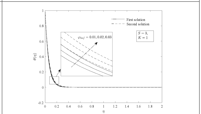
Figure 16: \theta(\eta) for varies \varphi_{hnf}
