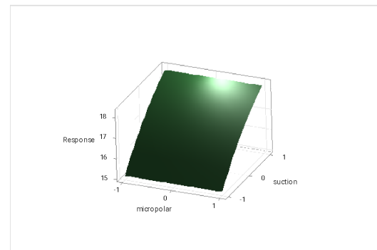
Figure 17: The interaction effect of hybrid nanoparticle, micropolar and suction on Nu_x Re_x^{-1/2}
