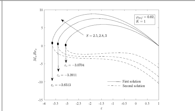
Figure 3: M_w Re_x for different S
