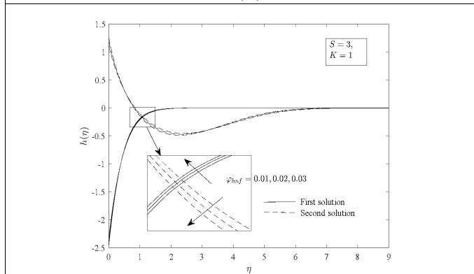
Figure 15: h(\eta) for varies \varphi_{hnf}
