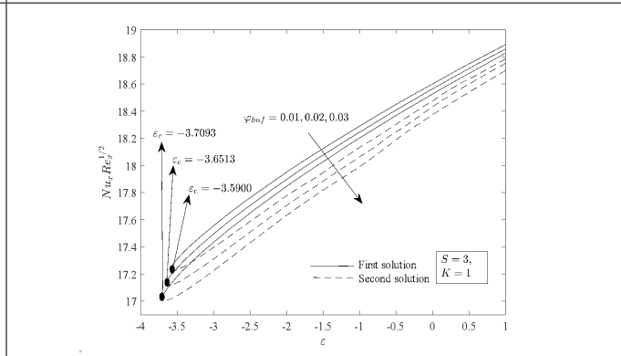
Figure 7: Nu_x Re_x^{-1/2} for different S
